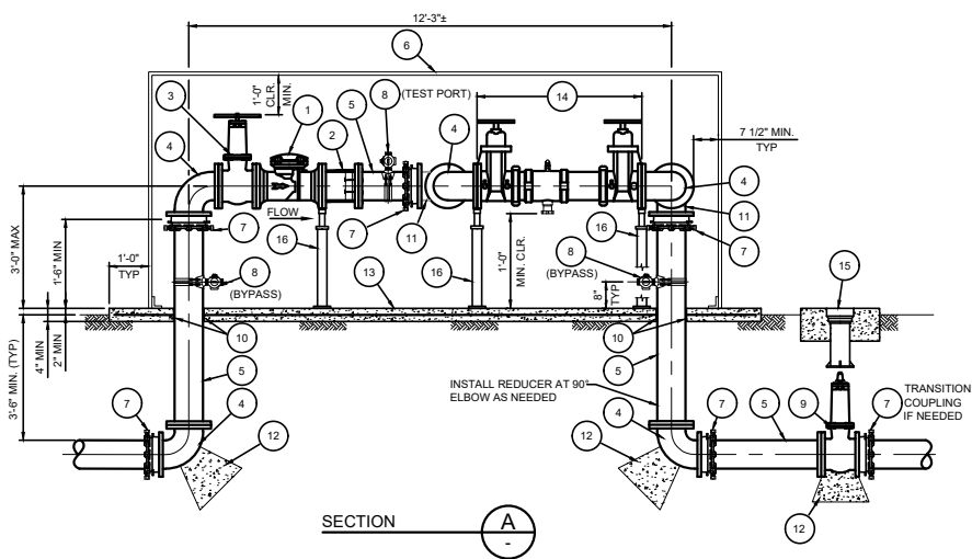
8" METER WITH DUAL 8" COLT 400 REDUCED PRESSURE PRINCIPLE ASSEMBLY SCALE: 1/2" = 1'-0" (USE NRS GATE VALVES ONLY)
