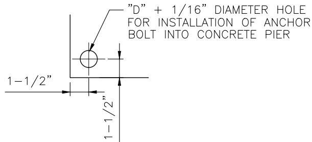
DETAIL "A"
