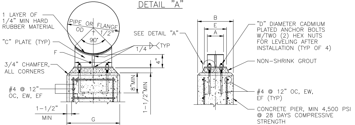
FRONT VIEW
