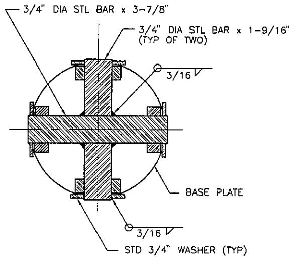
JOINT CROSS
