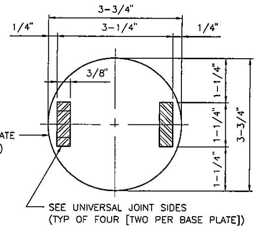
BASE PLATE
