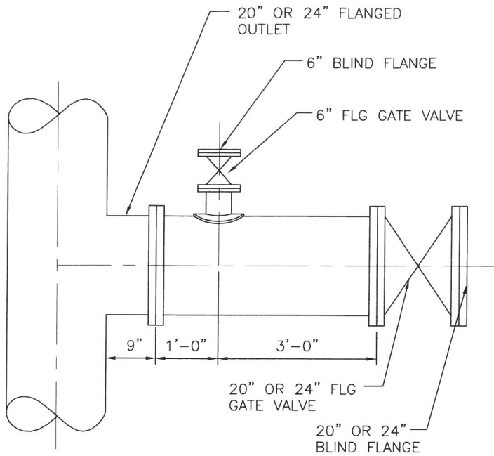
MCLP INSTALLATION
