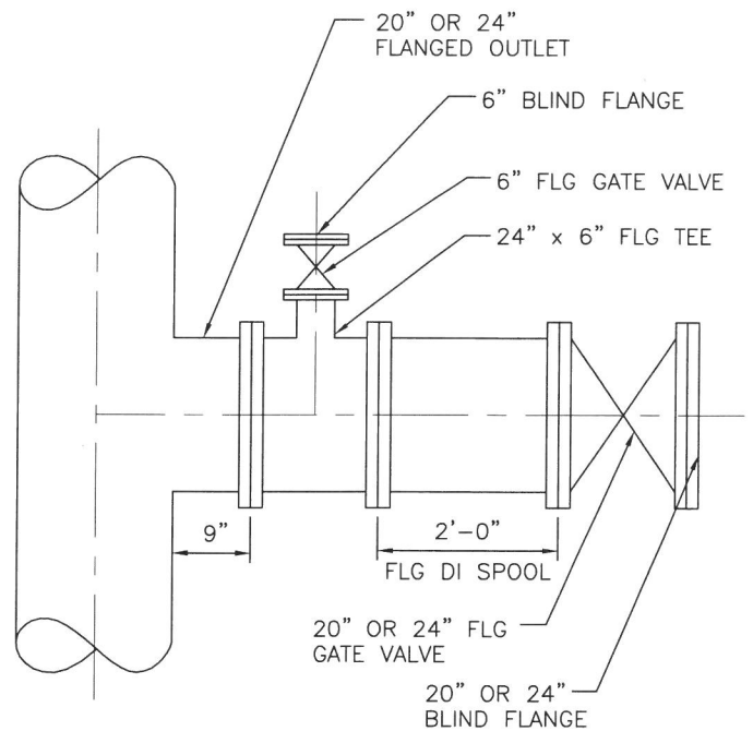
DIP INSTALLATION
