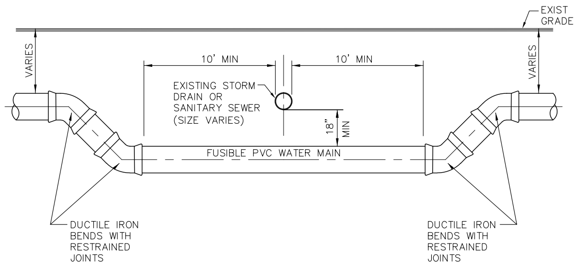
FUSIBLE PVC PIPE OPTION
