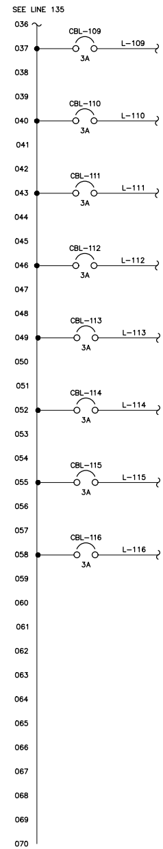
2-13 SLOT PLC RACK - 120VAC POWER DISTRIBUTION SCHEMATIC
