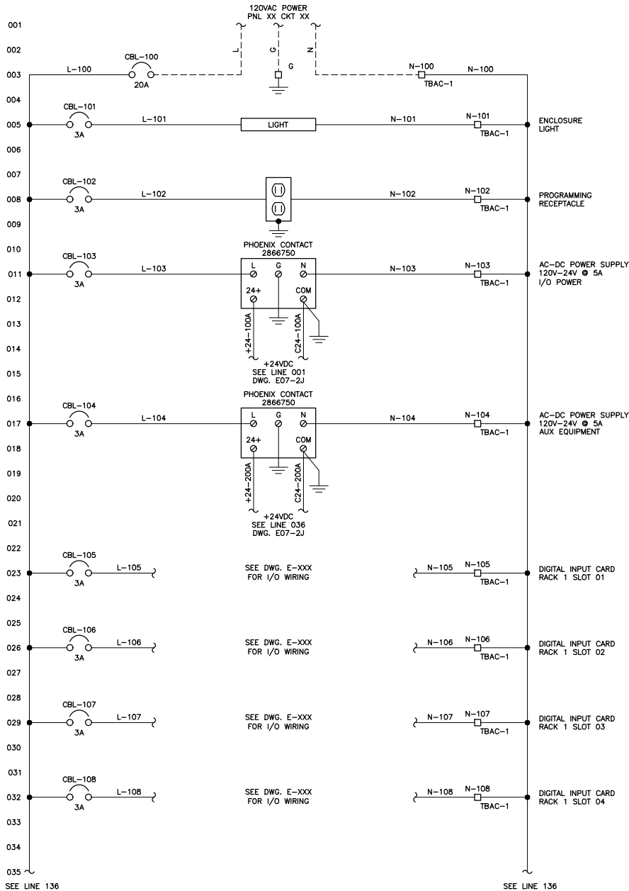
2-13 SLOT PLC RACK - 120VAC POWER DISTRIBUTION SCHEMATIC
