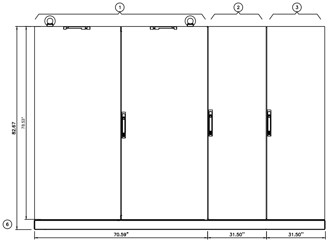
EXTERIOR LAYOUT – FRONT ACCESS SHOWN WITH COMMUNICATIONS CABINET
