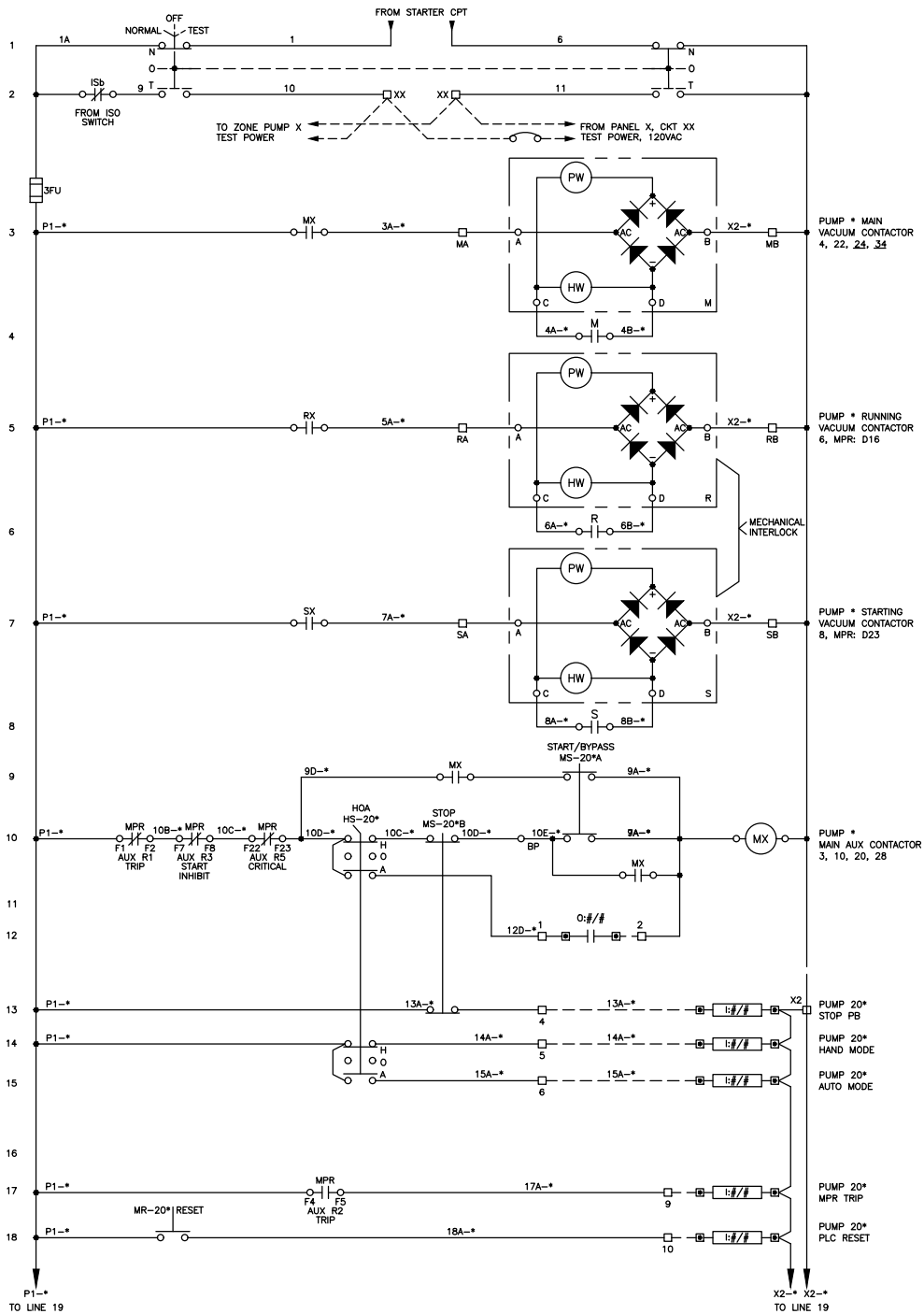
TYPICAL RVAT MOTOR STARTER WITH GE 469 MPR FOR 400 - 900 HP AT 4160 VOLTS, 3 DIA, 60HZ SCHEMATIC DIAGRAM II
