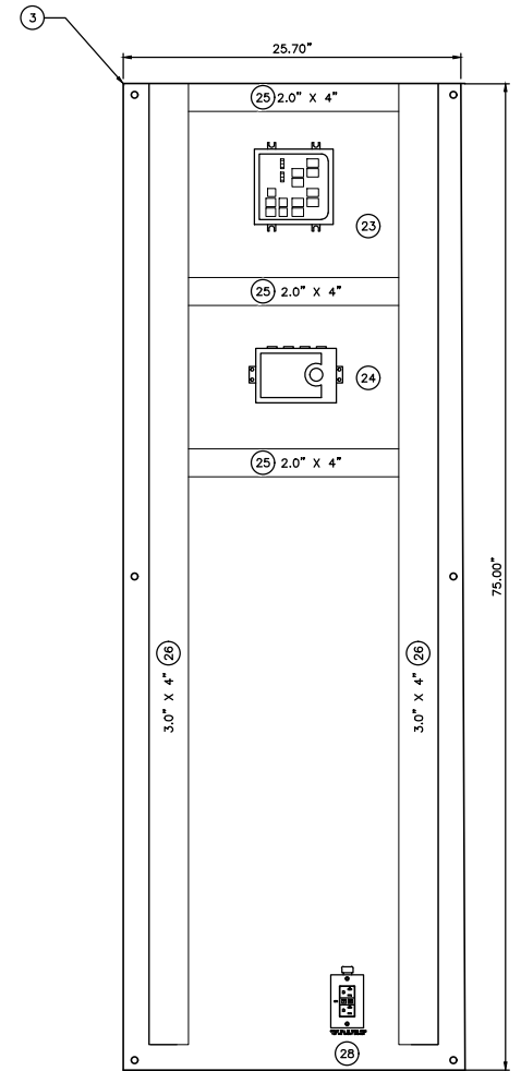
BACKPANEL LAYOUT – RIGHT SIDE
