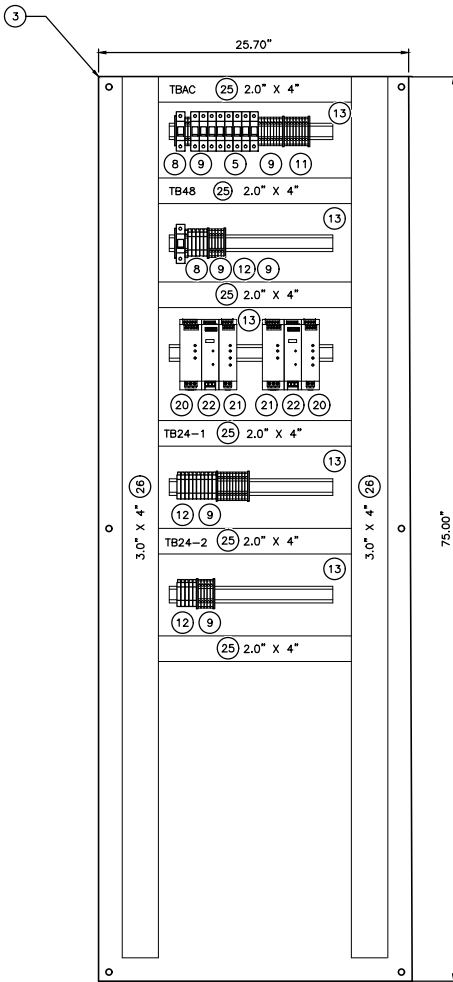
BACKPANEL LAYOUT – LEFT SIDE
