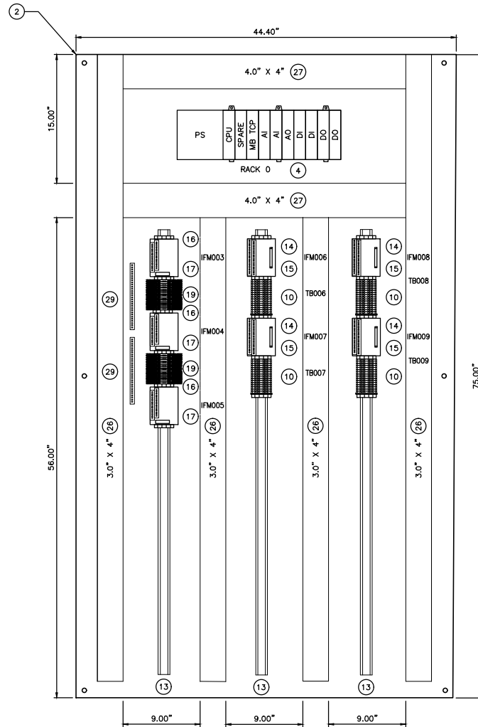
BACKPANEL LAYOUT – FRONT ACCESS
