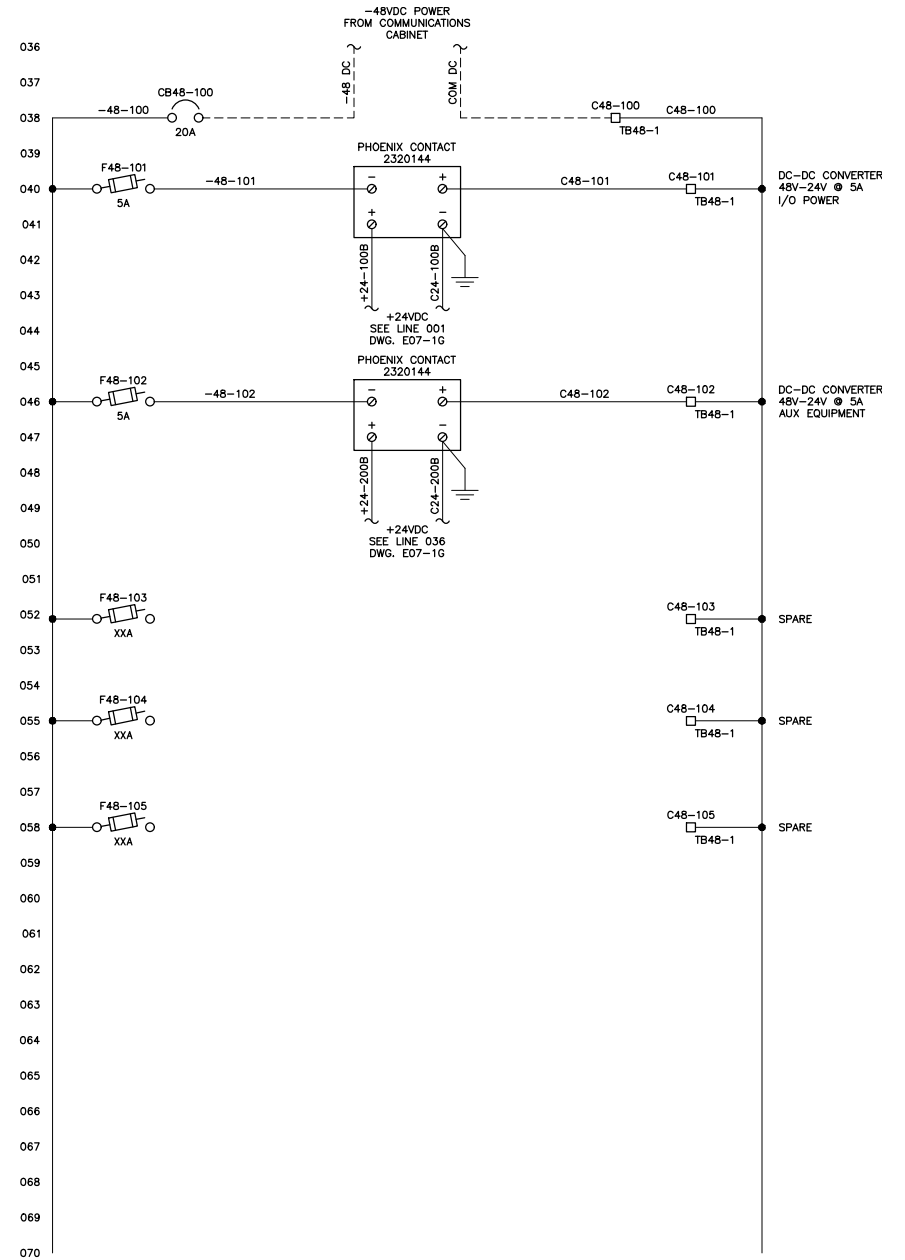
10 SLOT PLC RACK - 120VAC & 48VDC POWER DISTRIBUTION W/AC SCHEMATIC
