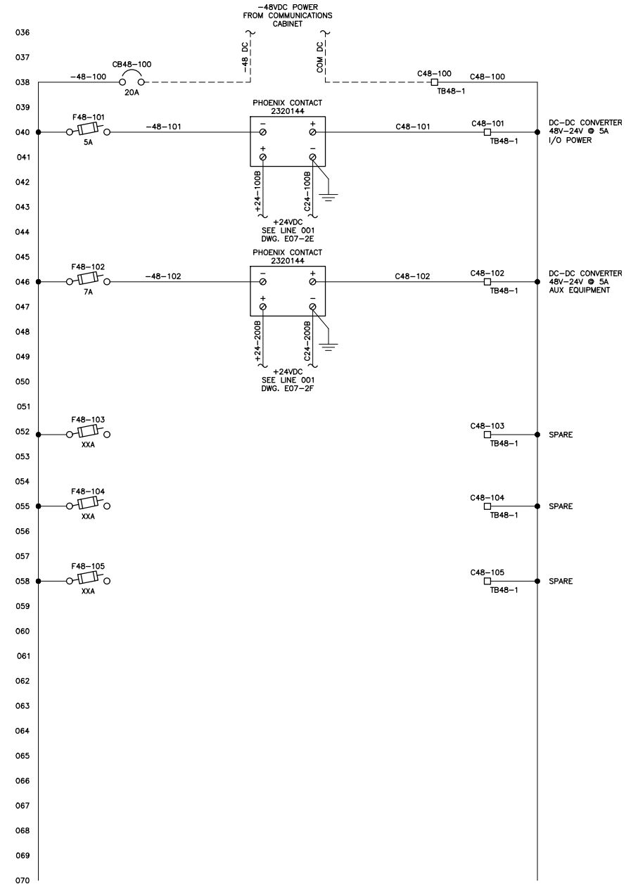
2-13 SLOT PLC RACK - 120VAC & 48VDC POWER DISTRIBUTION SCHEMATIC
