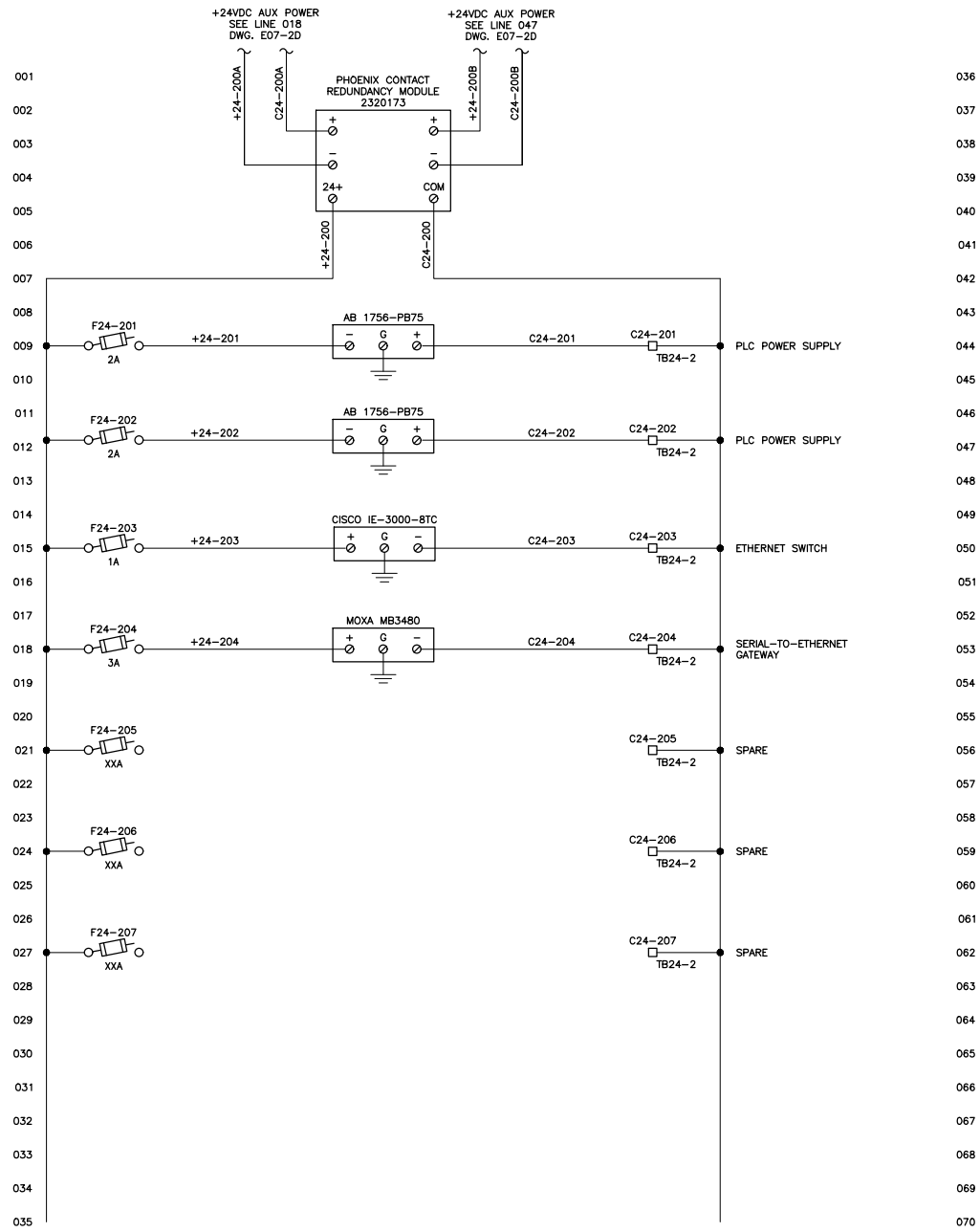
2-13 SLOT PLC RACK - 24VDC POWER DISTRIBUTION SCHEMATIC II NOT TO SCALE E07-2F 042121
