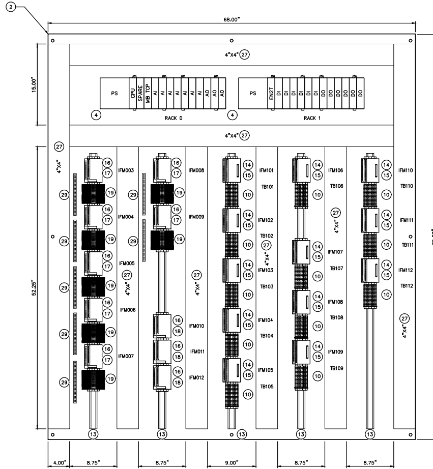
BACKPANEL LAYOUT - FRONT ACCESS
