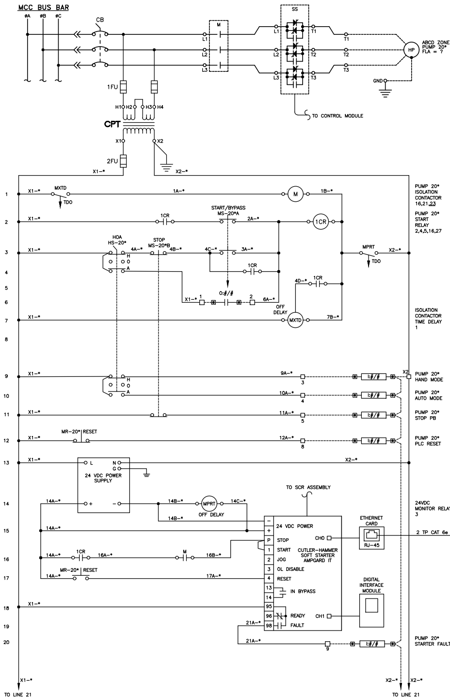
TYPICAL RVSS MOTOR STARTER FOR 100 - 300 HP AT 480 VOLTS, 3 DIA, 60HZ SCHEMATIC DIAGRAM
