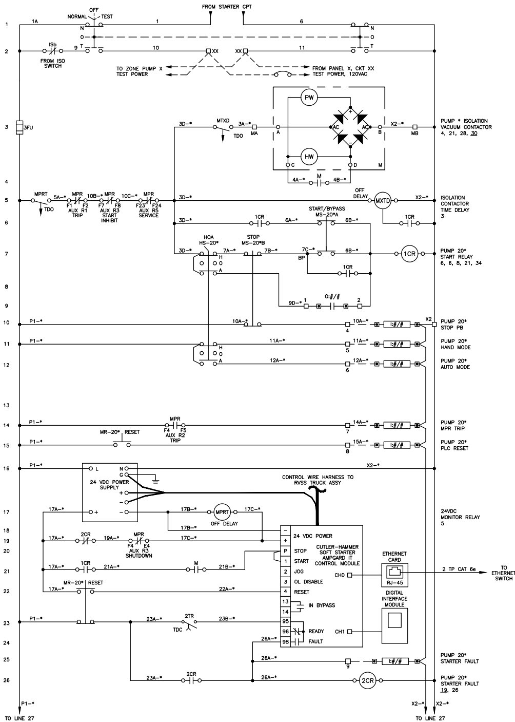
TYPICAL RVSS MOTOR STARTER WITH GE 469 MPR FOR 400 - 900 HP AT 4160 VOLTS, 3 DIA, 60HZ SCHEMATIC DIAGRAM II
