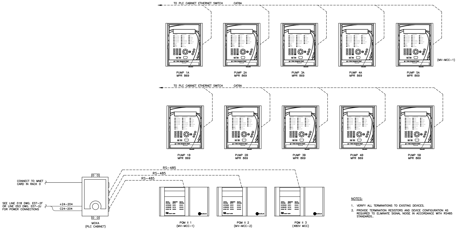
2-13 SLOT PLC ETHERNET / SERIAL NETWORK DIAGRAM NOT TO SCALE
