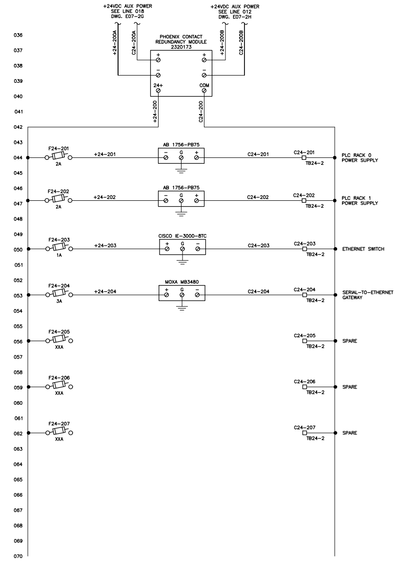
2-13 SLOT PLC RACK - 24VDC POWER DISTRIBUTION SCHEMATIC III NOT TO SCALE
