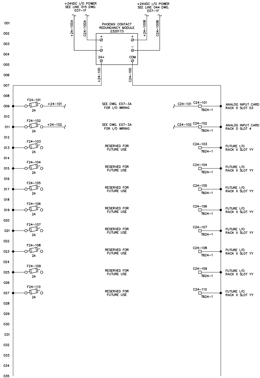
10 SLOT PLC RACK - 24VDC POWER DISTRIBUTION SCHEMATIC NOT TO SCALE E07-1G 042121
