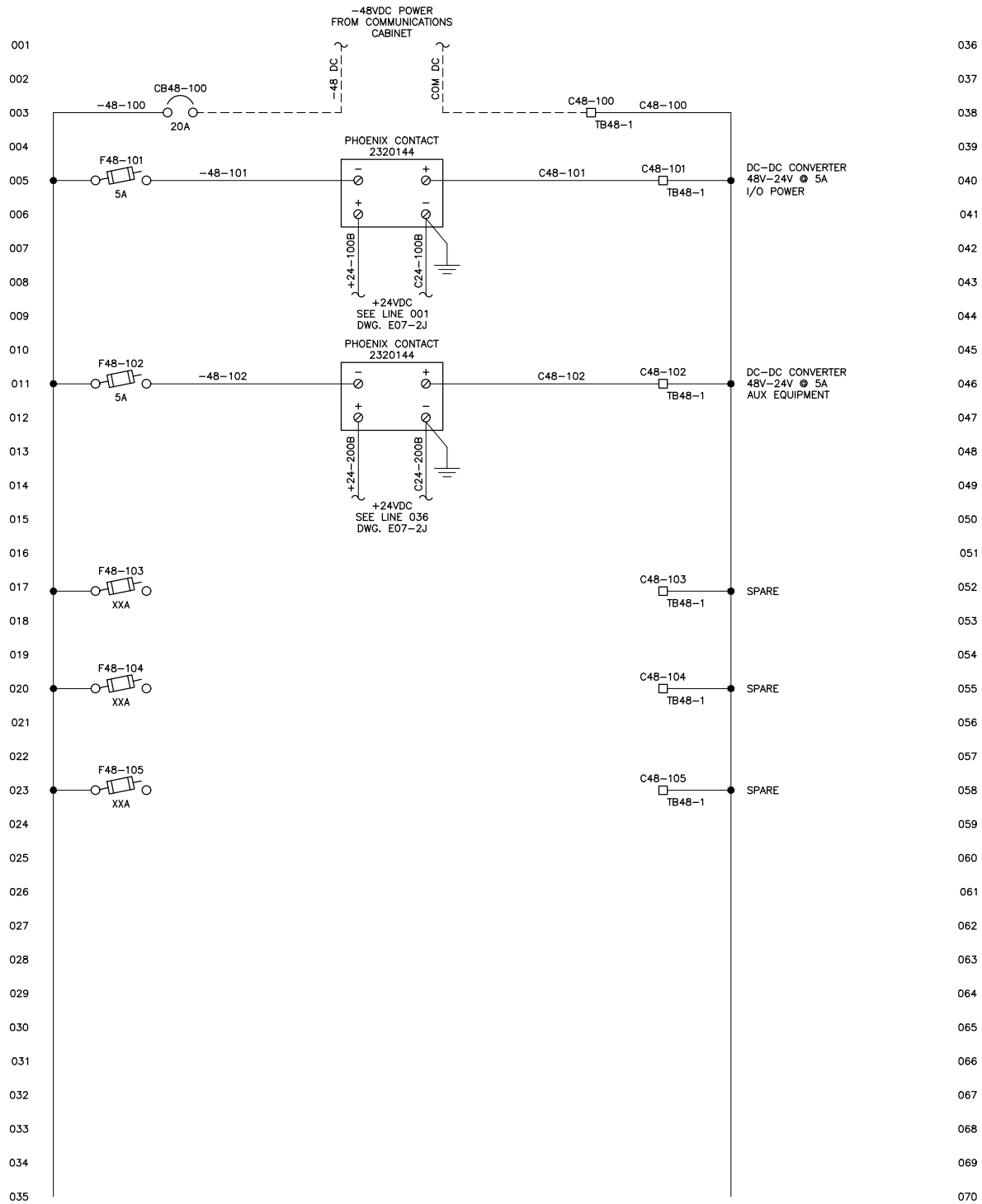
2-13 SLOT PLC RACK - 48VDC POWER DISTRIBUTION SCHEMATIC
