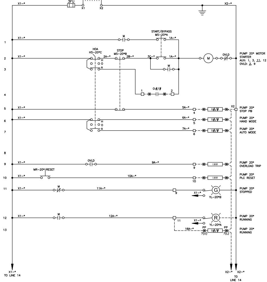
TYPICAL FVNR MOTOR STARTER WITH OLVD'S FOR 1/2 - 75 HP AT 480 VOLTS, 3 DIA, 60HZ SCHEMATIC DIAGRAM
