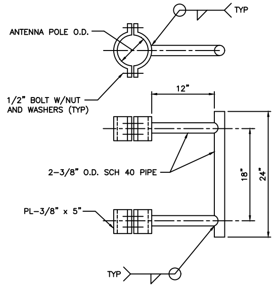
DETAIL "B"
