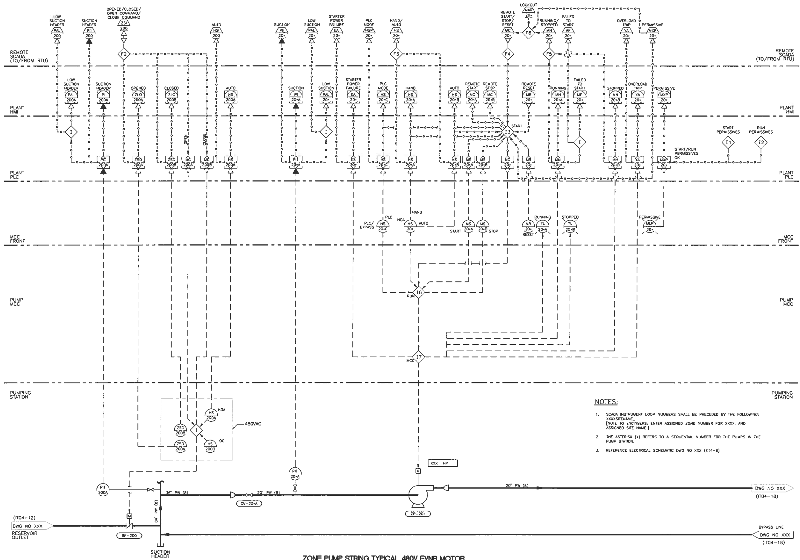
ZONE PUMP STRING TYPICAL 480V FVNR MOTOR STARTER PROCESS AND INSTRUMENTATION DIAGRAM NOT TO SCALE 1T04-13 041907
