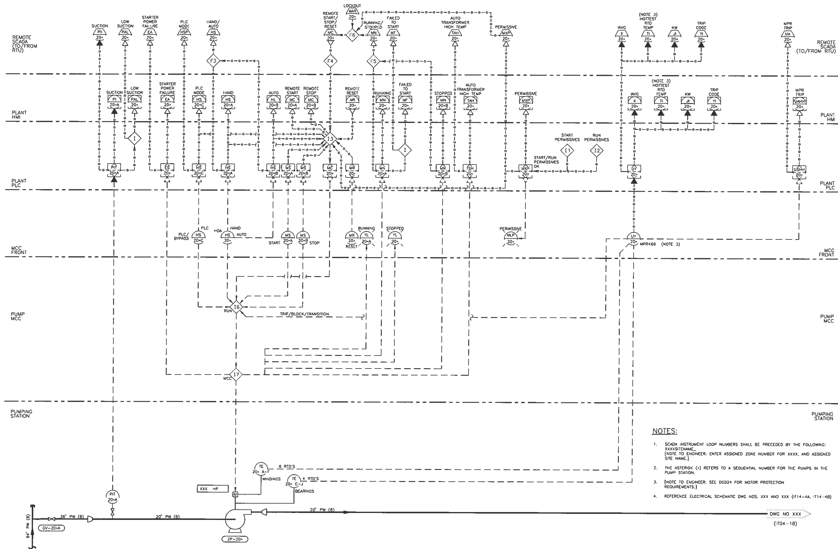
ZONE PUMP STRING TYPICAL 4160V RVAT MOTOR STARTER PROCESS AND INSTRUMENTATION DIAGRAM
