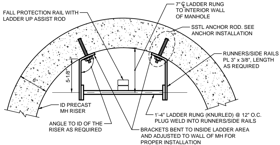
LADDER IN MANHOLE
