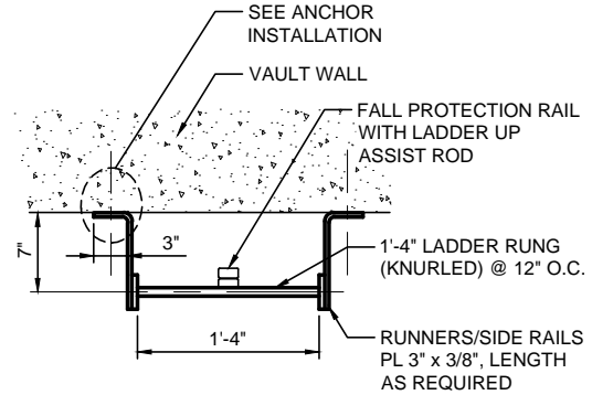
LADDER IN VAULT
