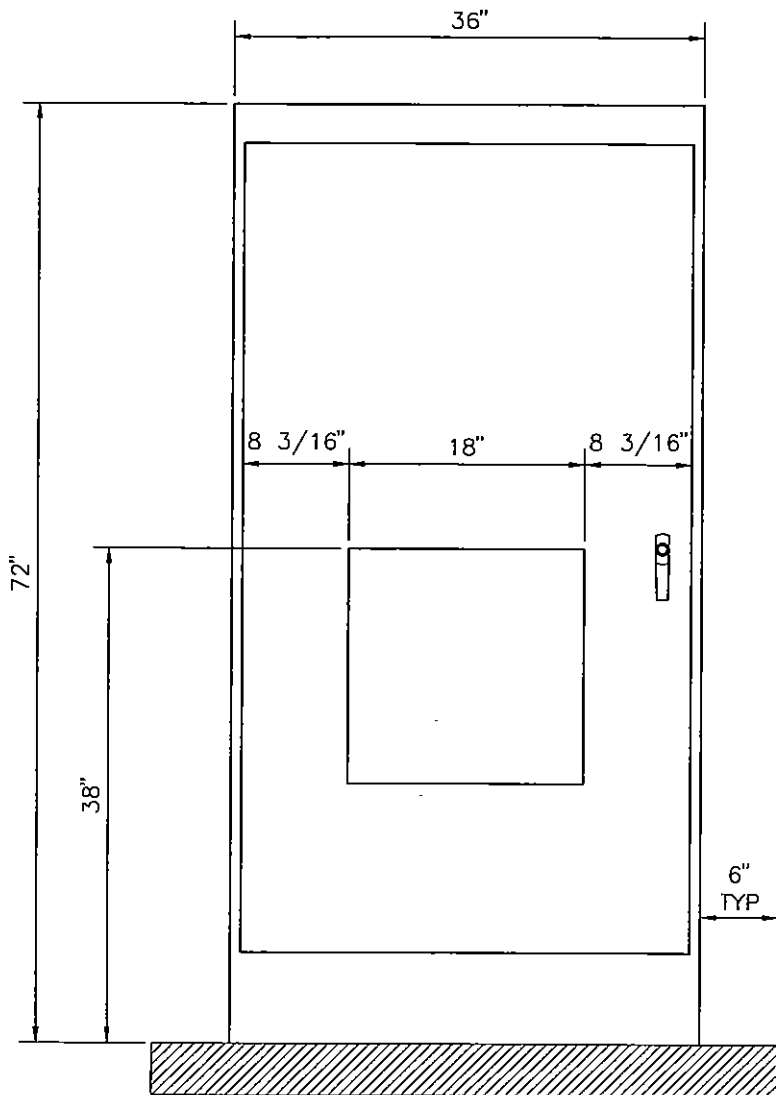
FRONT VIEW OF PLC ENCLOSURE
