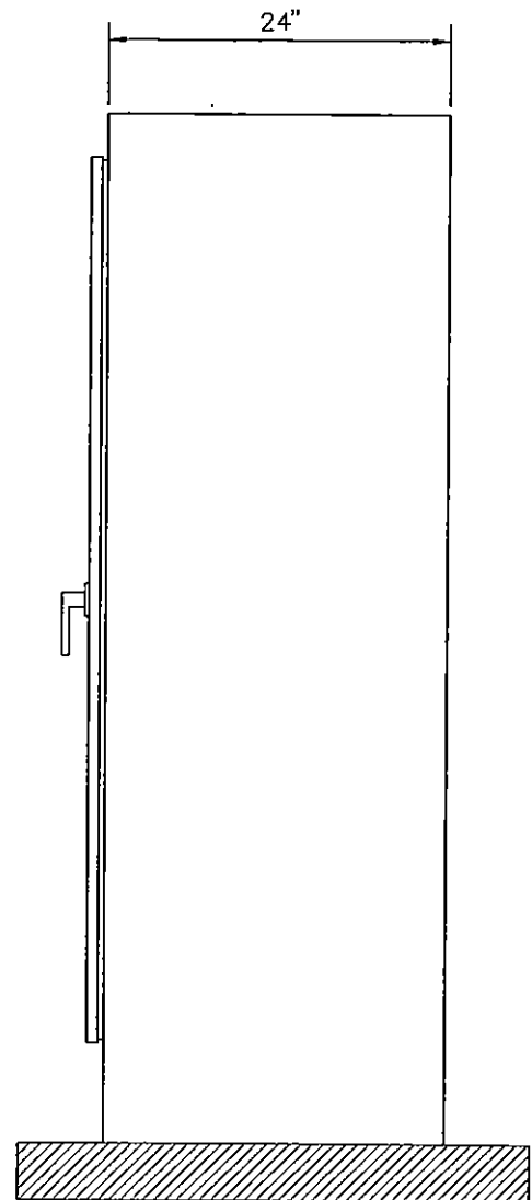
SIDE VIEW OF PLC ENCLOSURE
