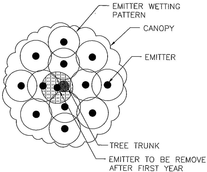
EMITTER LAYOUT (FIRST YEAR)
